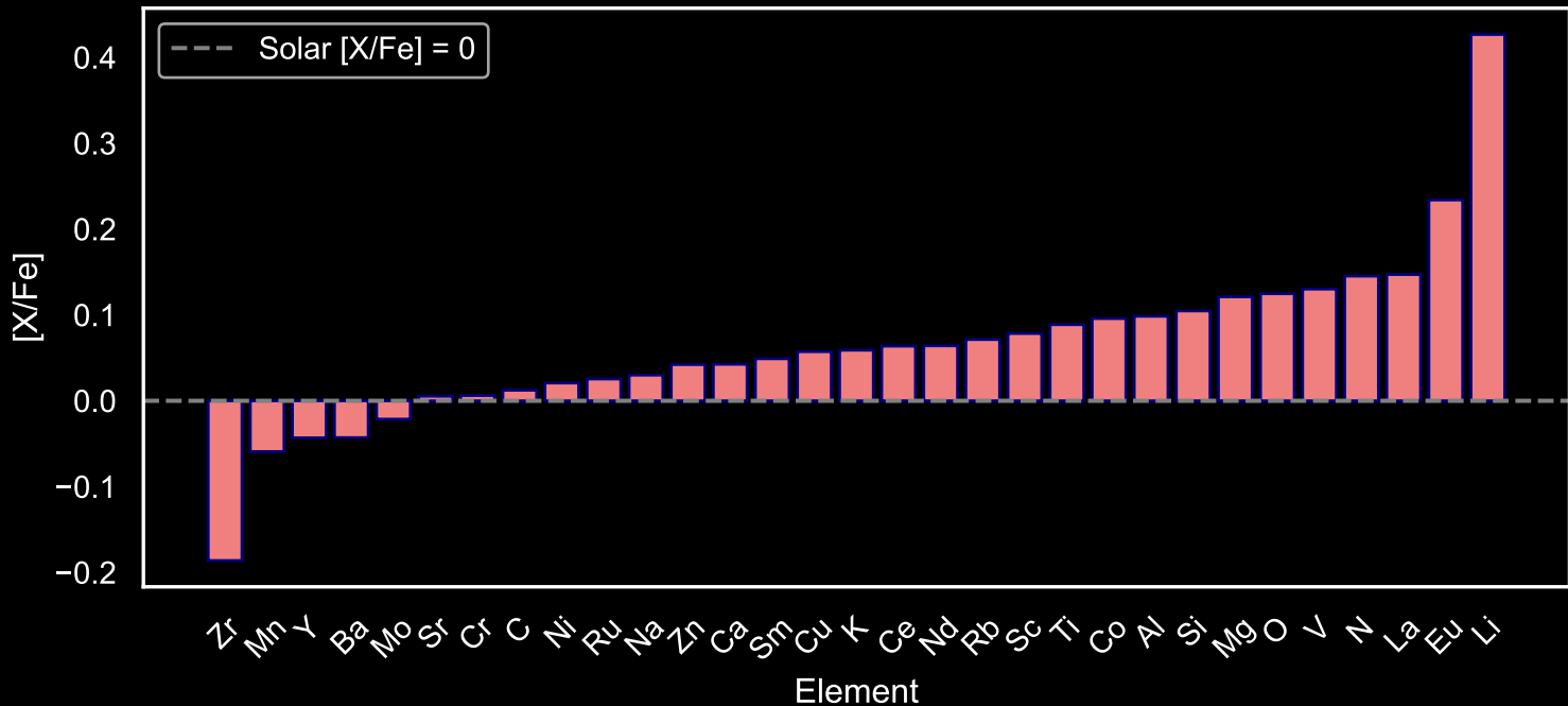
Abundance Pattern for GALAH Star Field [78] (N=221)
