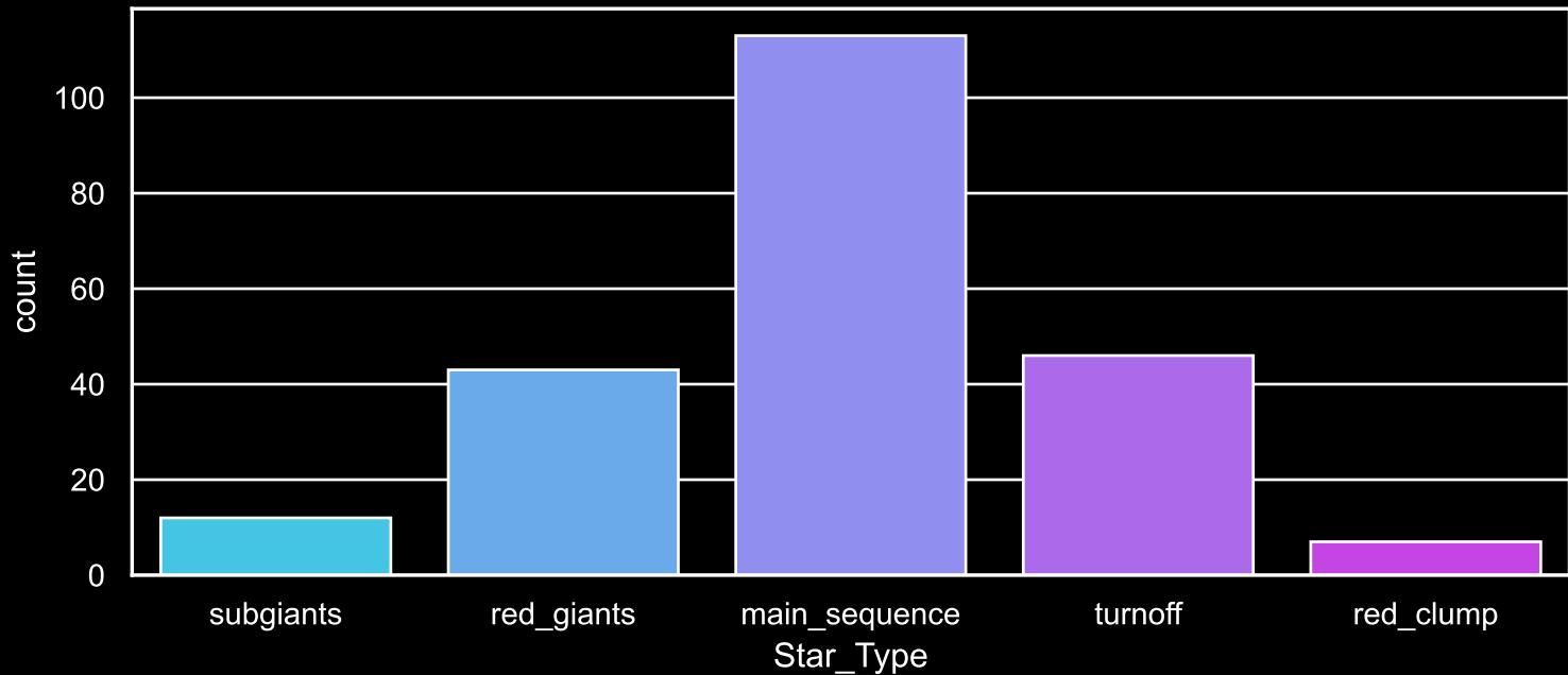
Field [78] Count plot of Star Type
