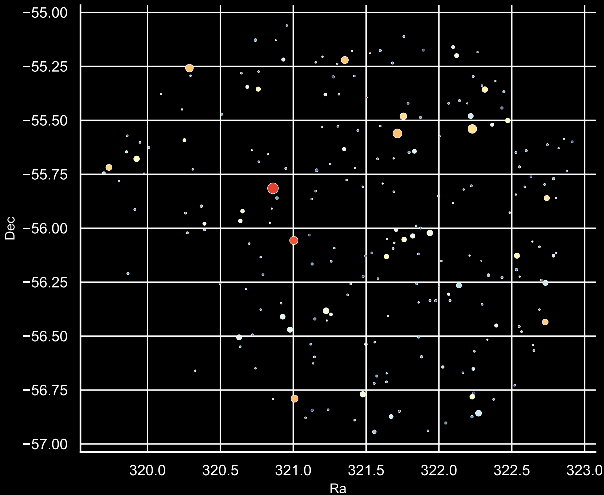
Field [78] Ra [321.55] Dec [-55.98] Stars: 221
