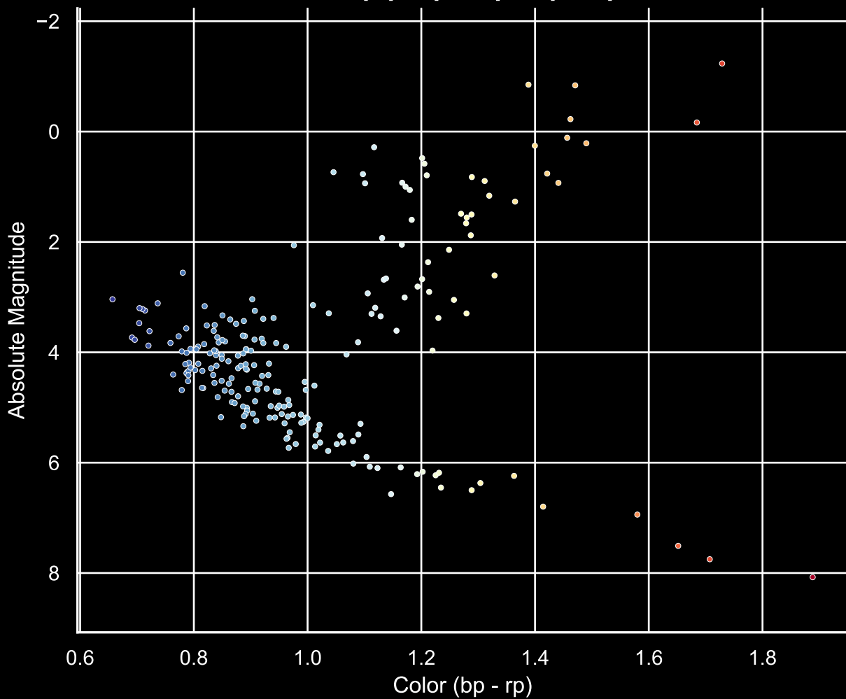
GALAH Hertzprung-Russel Diagram Field [78] Ra [321.55] Dec [-55.98]
