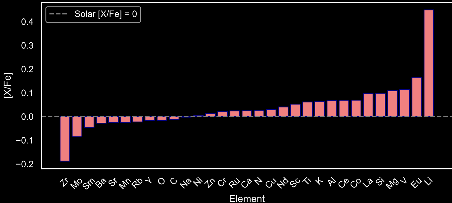
Abundance Pattern for GALAH Main Sequence Stars: Star Field [78] (N=113)
