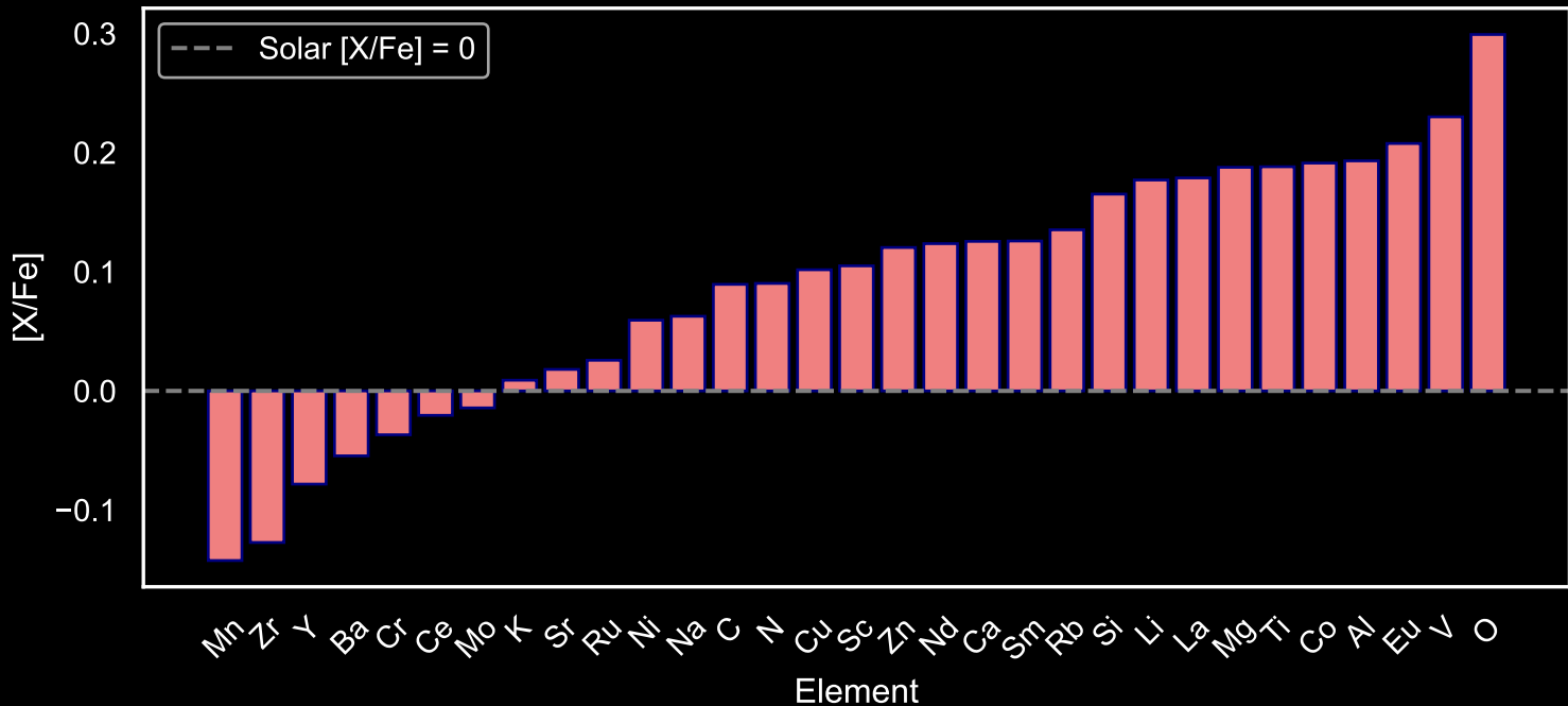
Abundance Pattern for GALAH Red Giants: Star Field [78] (N=50)
